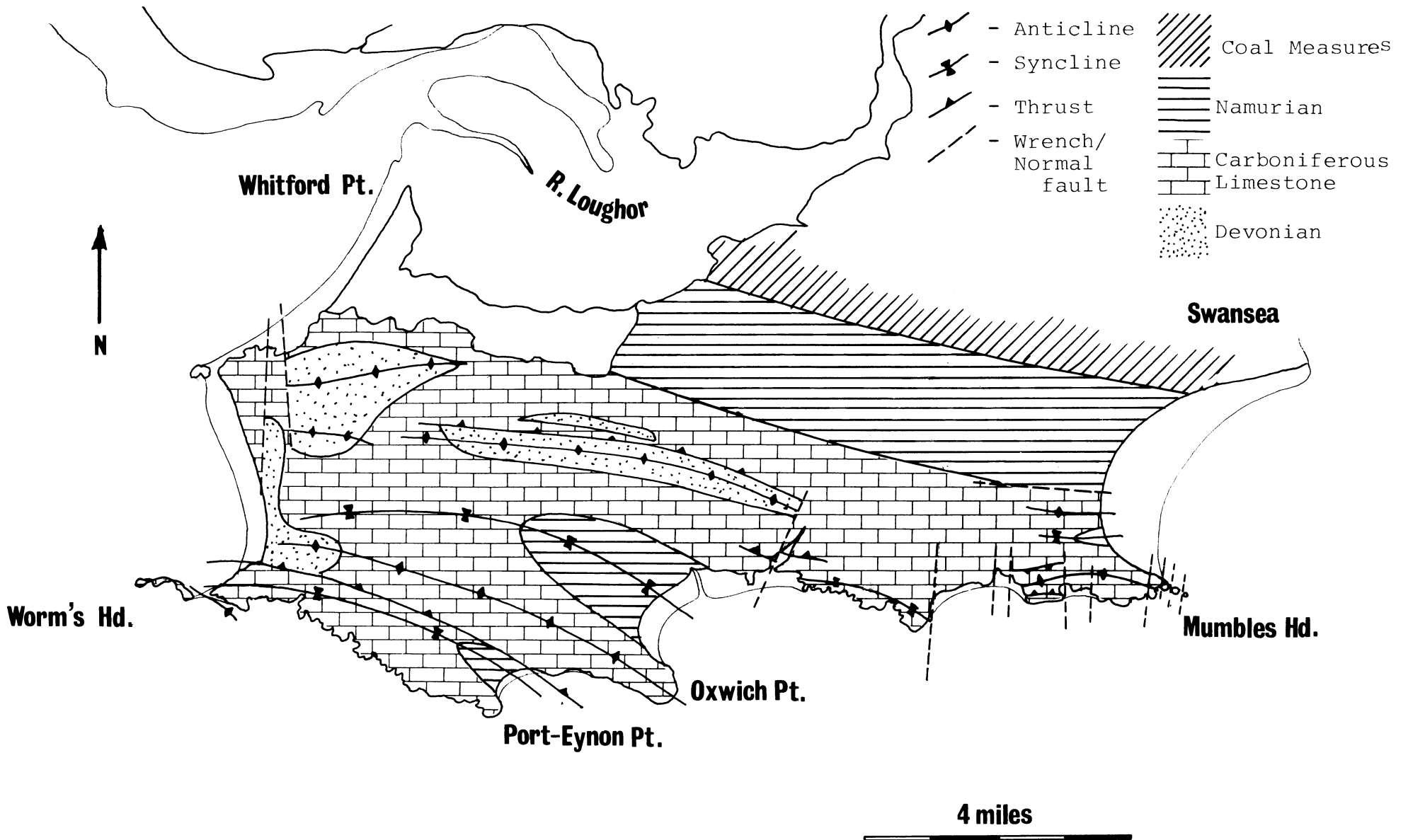
Fig. I GEOLOGICAL SKETCH - MAP of GOWER
